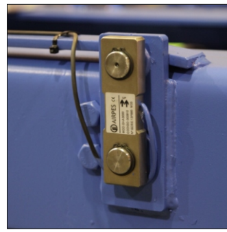
2 Overload limiter
